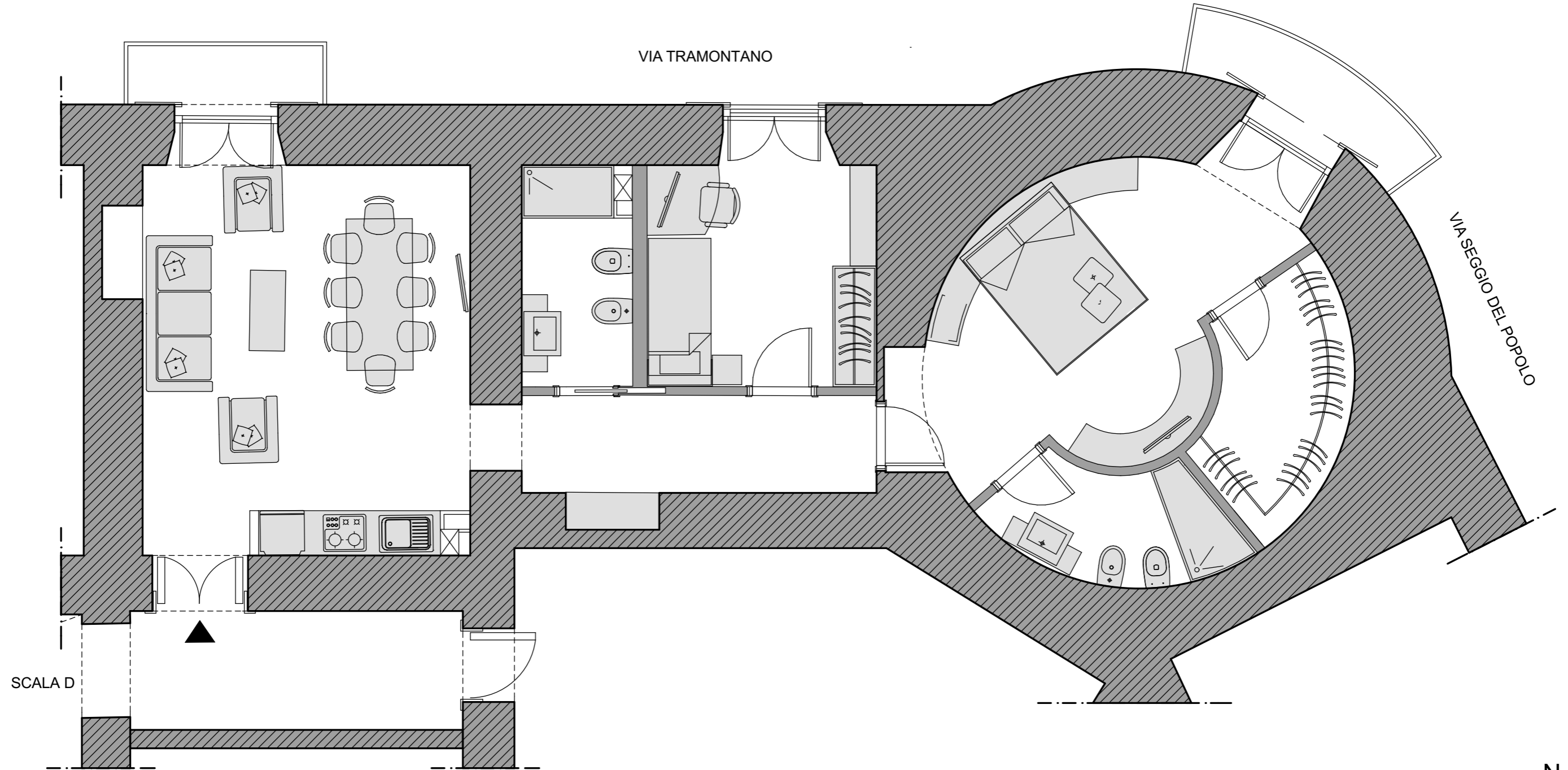
KEYPLAN
