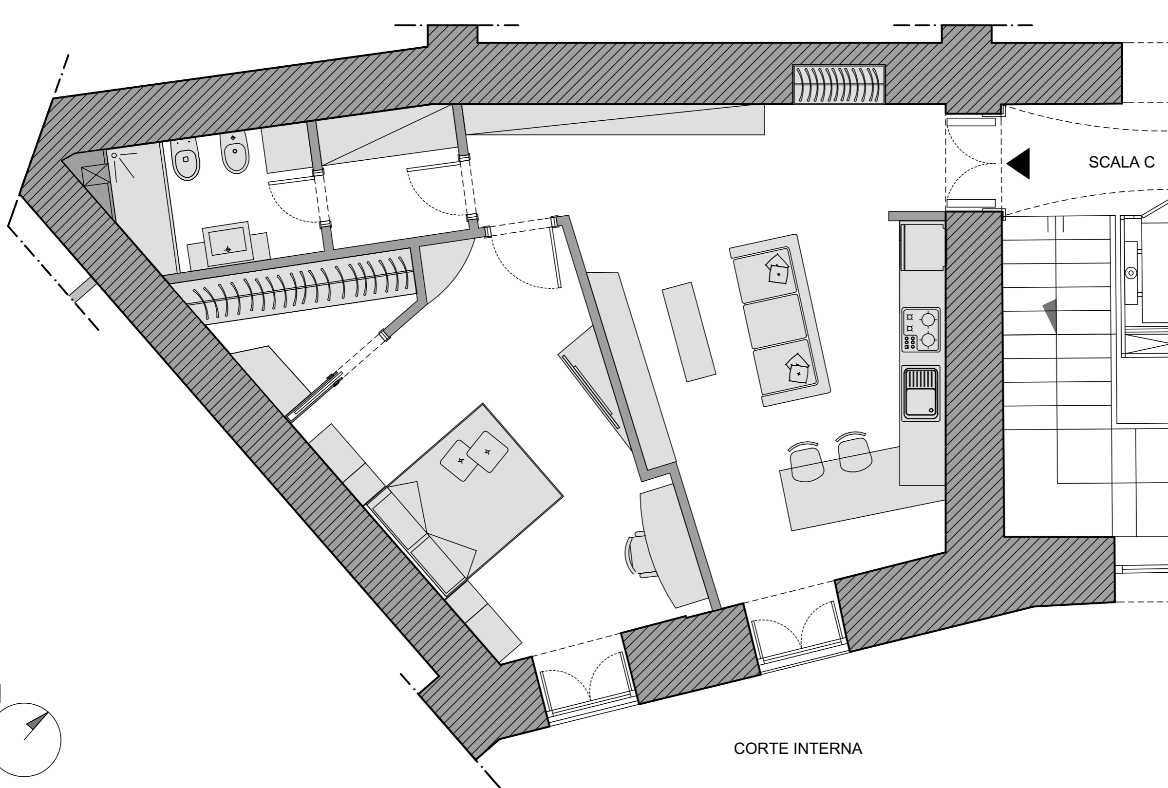
KEYPLAN
